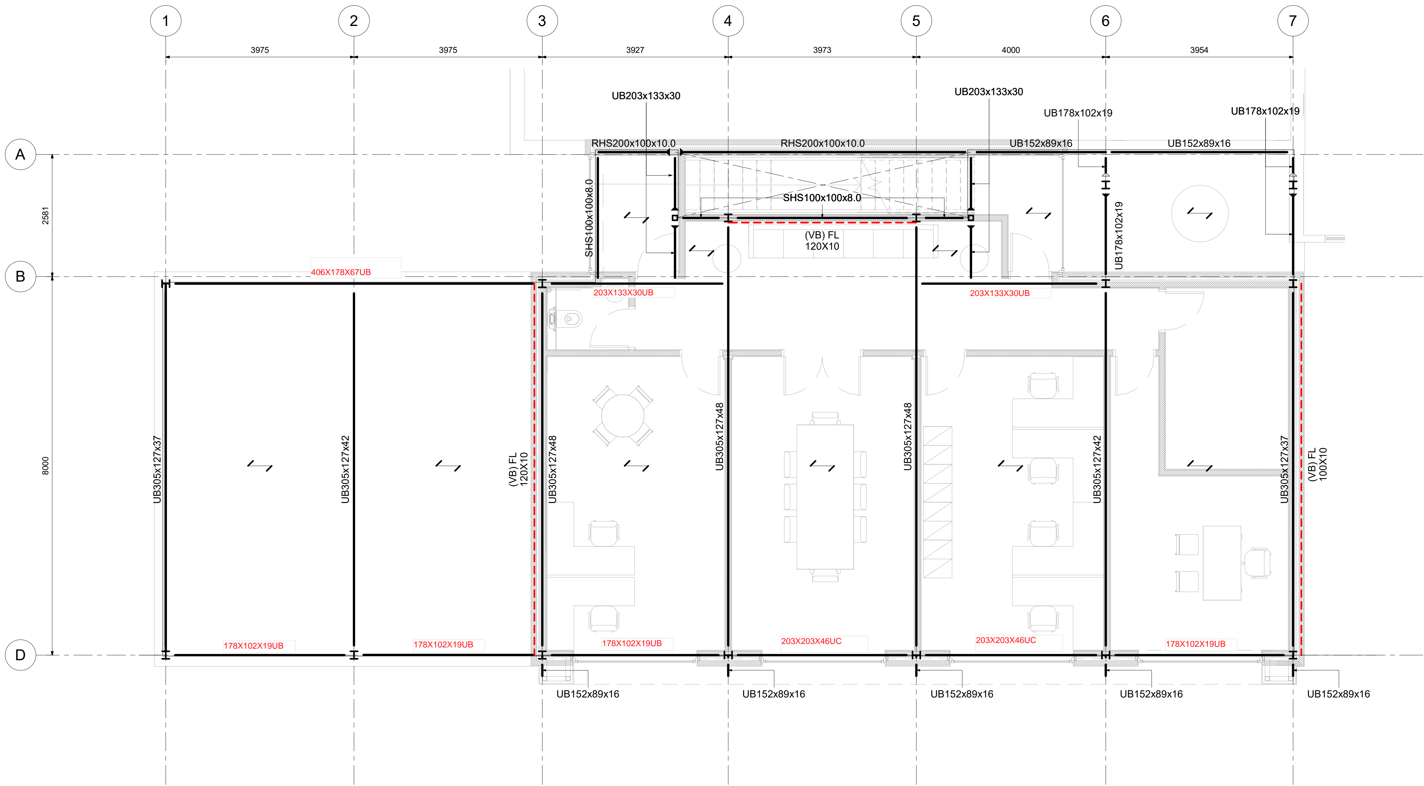
1: Plan - First Floor 1 : 50
