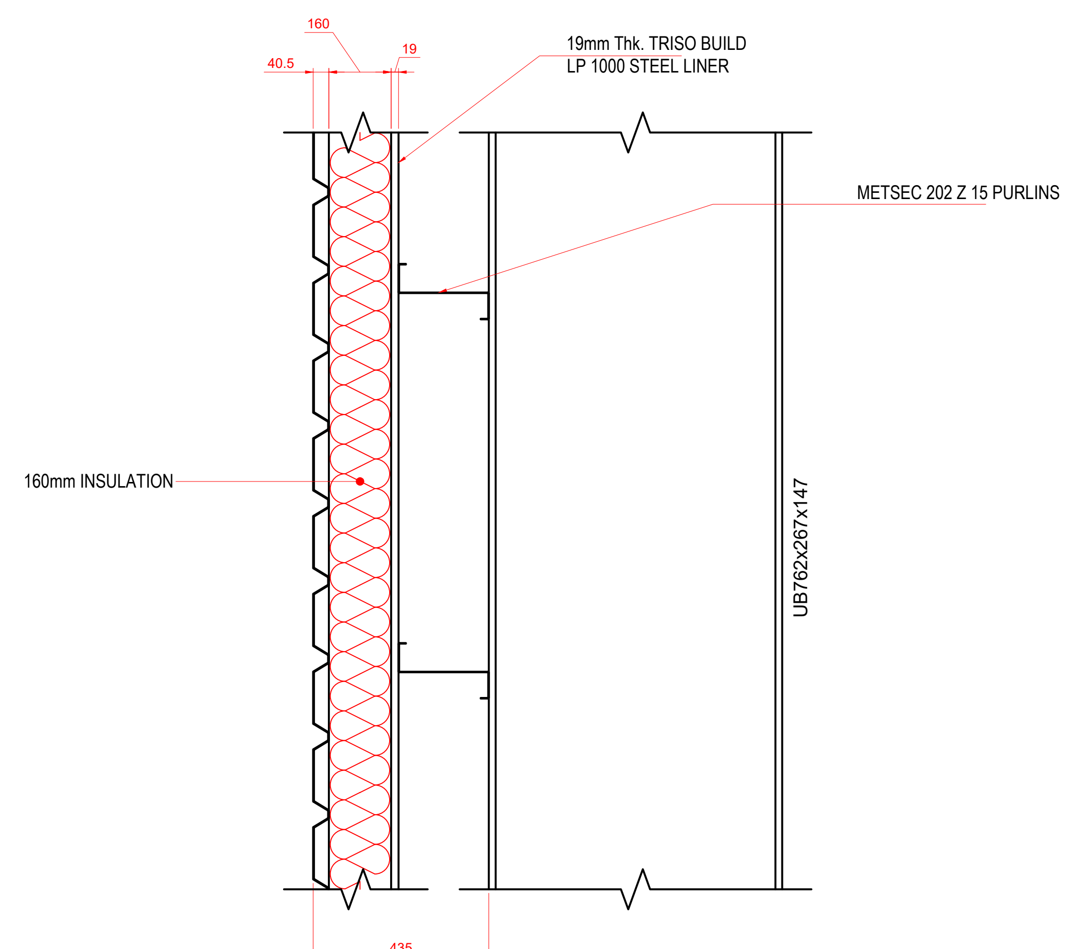
DETAIL - 2 SECTION THRU CLADDING SCALE 1:10
