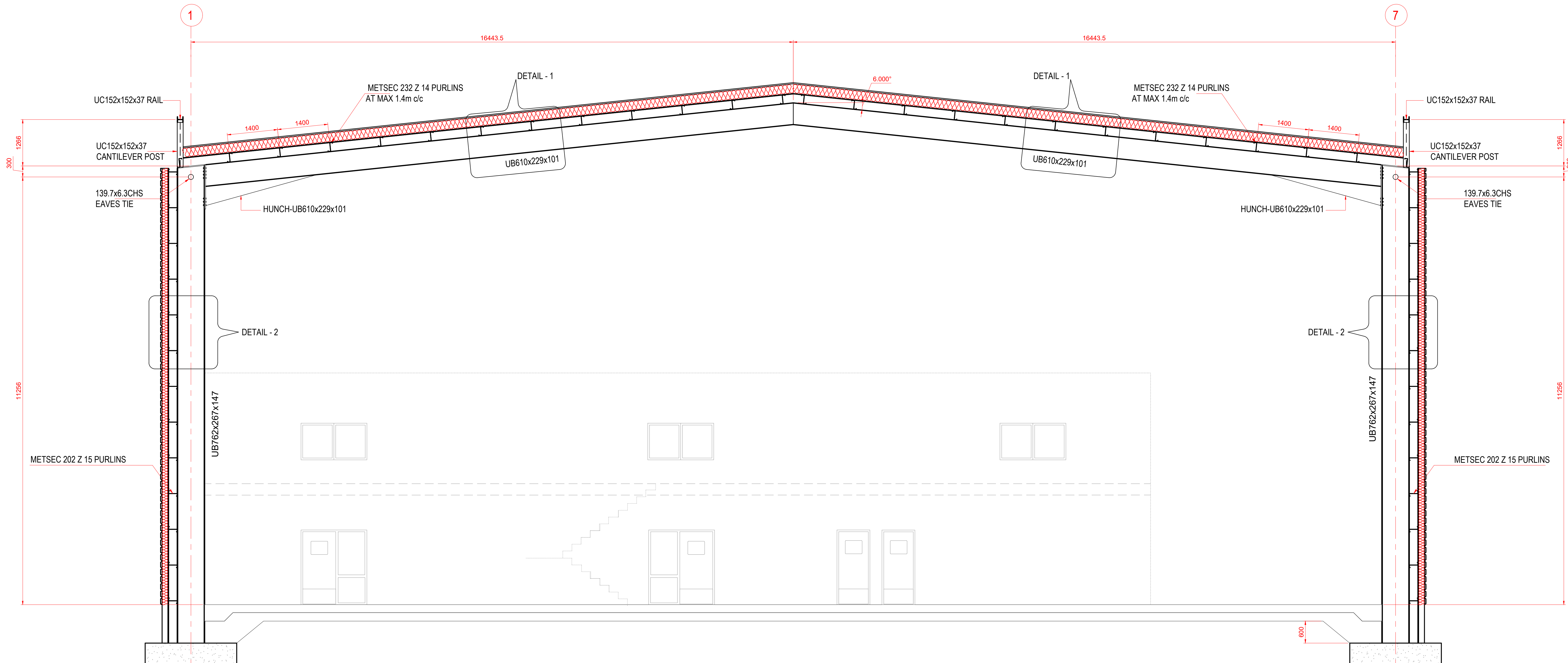
SECTION A-A SCALE 1:50
