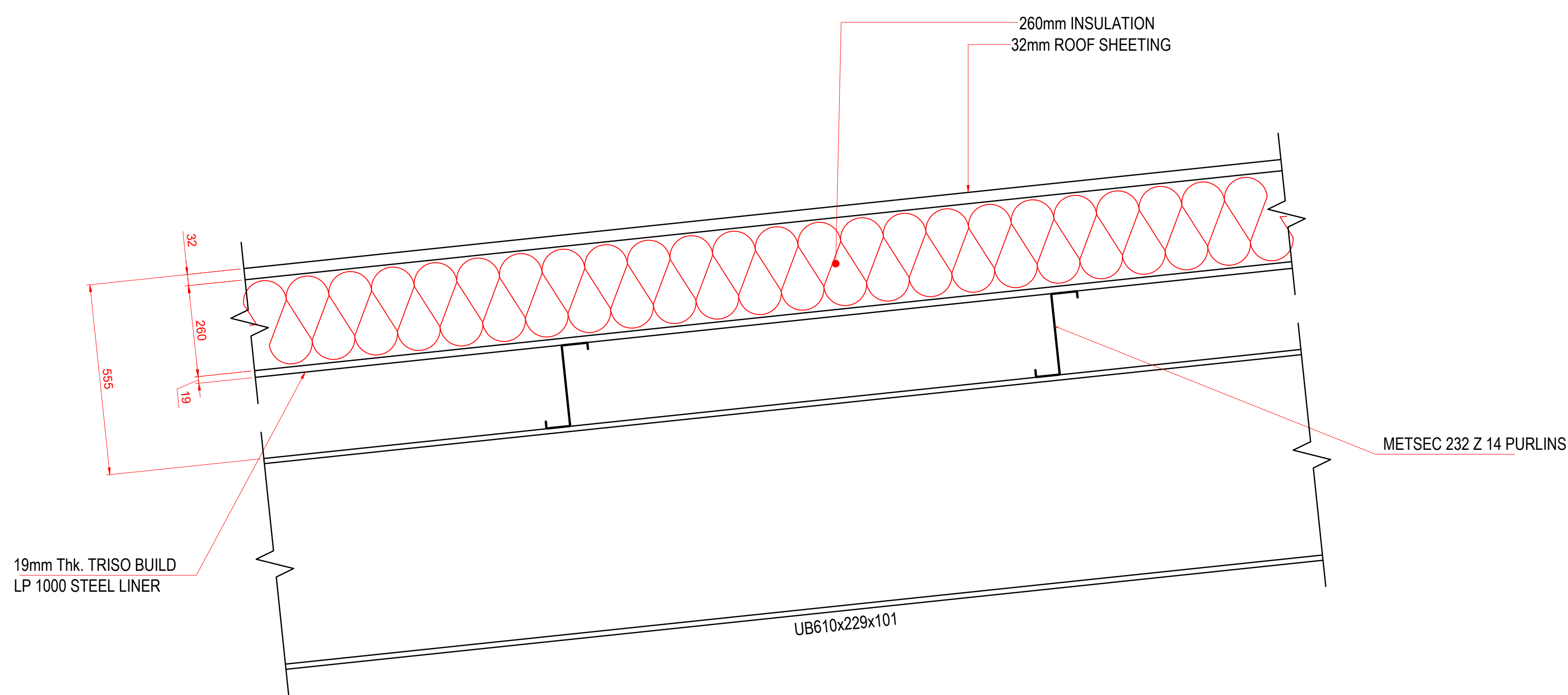
DETAIL - 1 SECTION THRU ROOF SCALE 1:10
